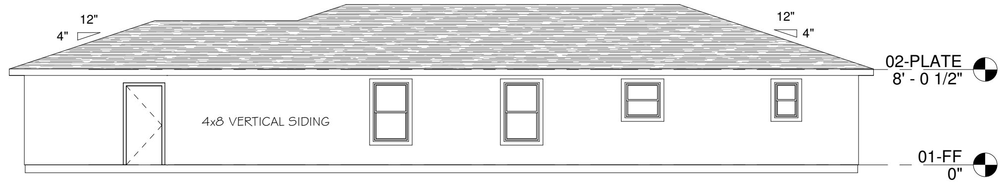
4 Rear - Single Garage 1/8" = 1'-0"
