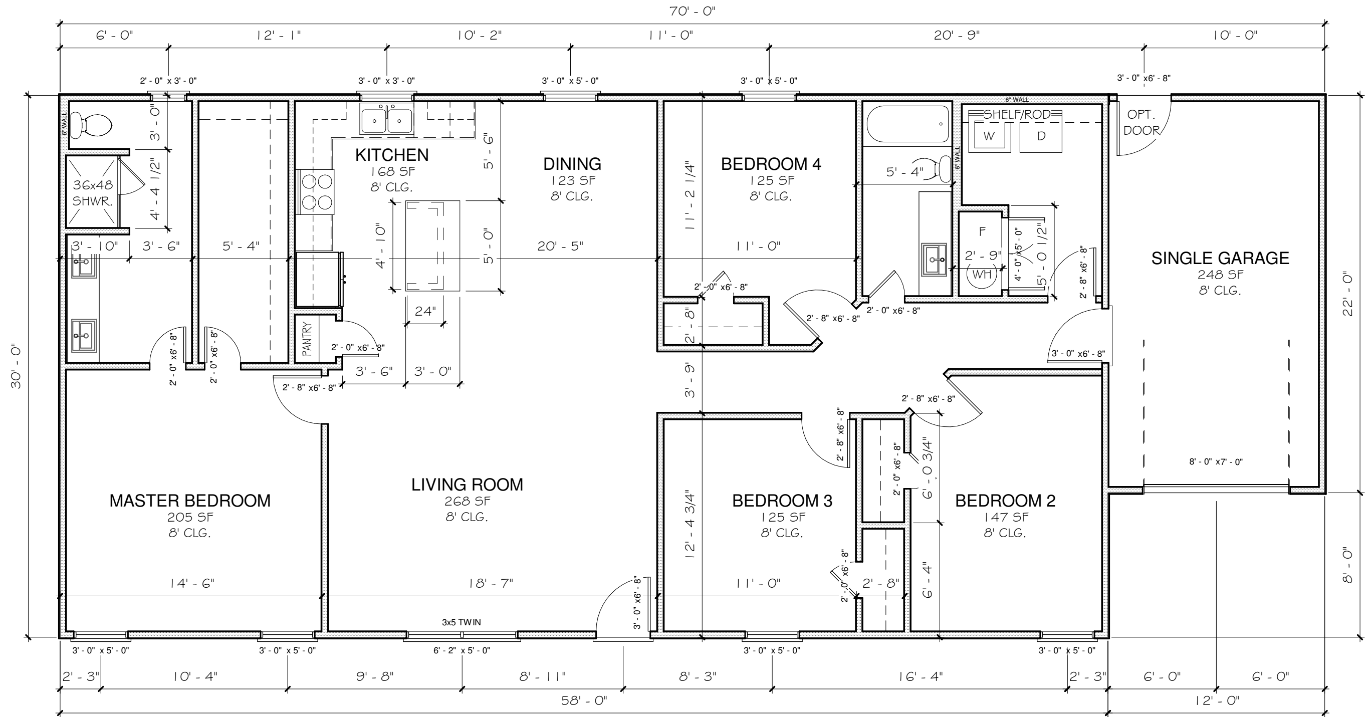
1 Floor Plan - Single Garage 3/16" = 1'-0"
